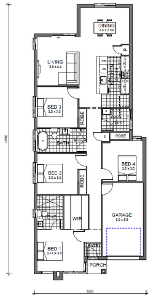
GROUND FLOOR
